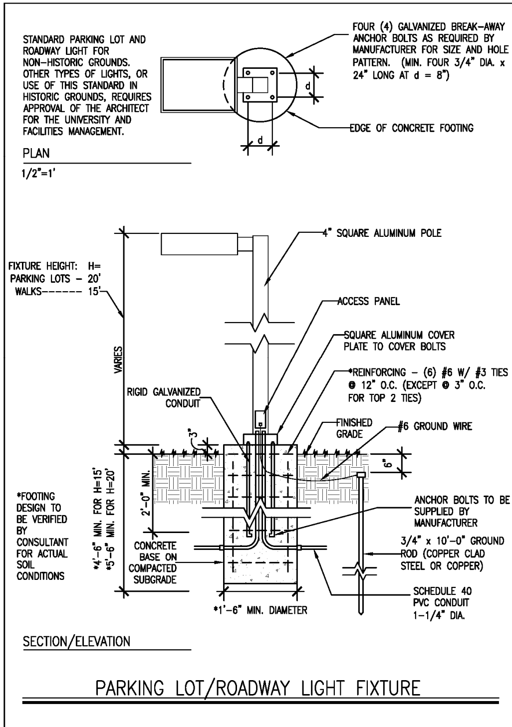
Figure 7: Parking Lot / Roadway Light Fixture
