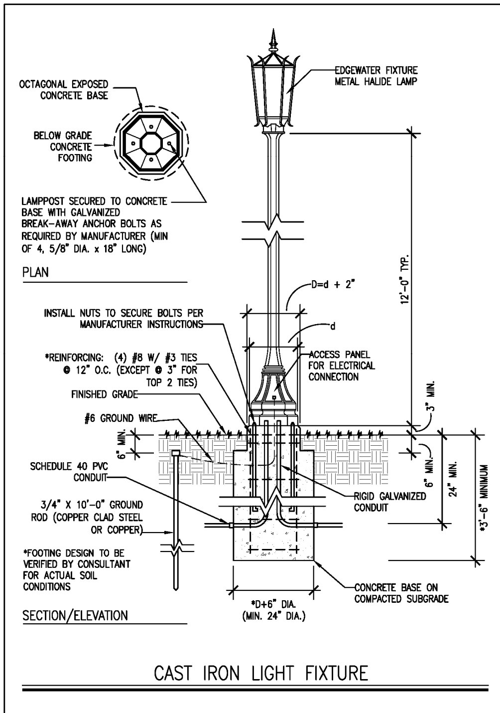
Figure 6: Cast Iron Light Fixture
