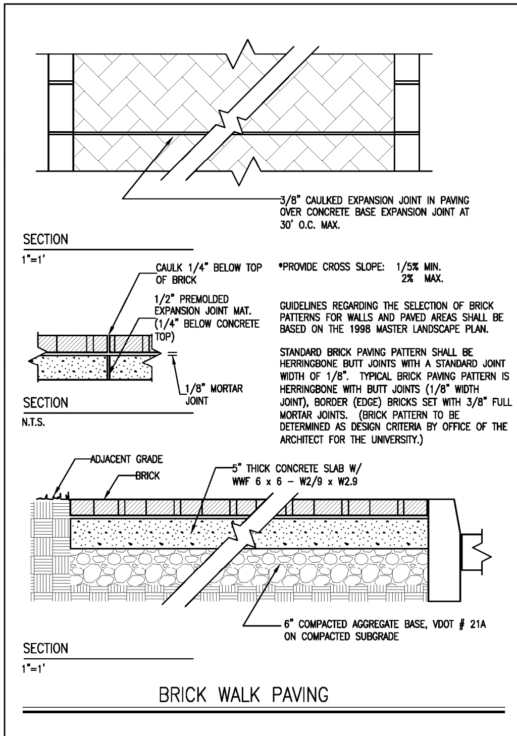
Figure 10: Brick Walk Paving
